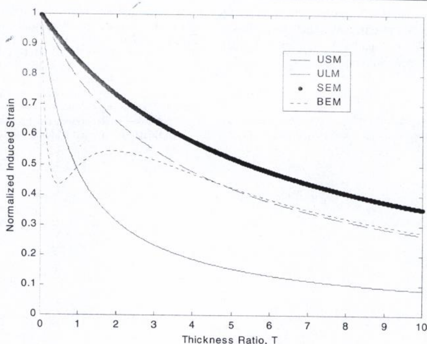
Figure 2. The relation between the normalized induced strain and the thickness ratio.
