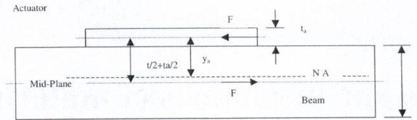
Figure 1. An actuator bonded to a one-dimensional beam.
